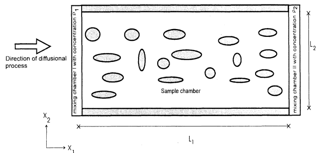
FIG. 1. Experimental setup for the estimation of effective diffusivities.
